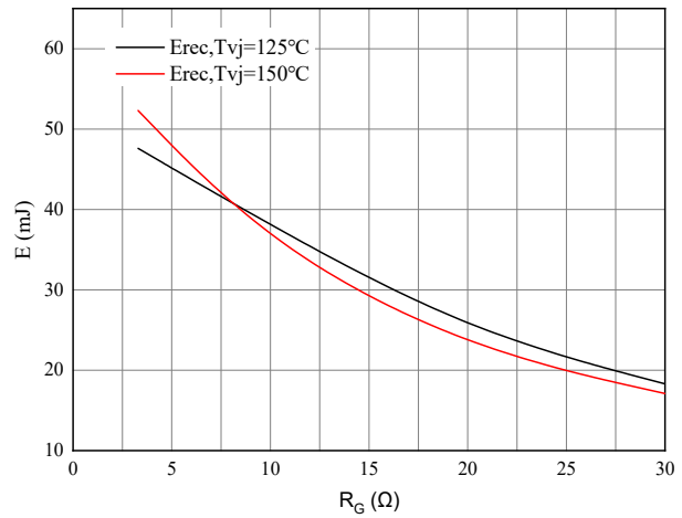
Figure 8. Switching losses of Diode I_F=300A , V_{CE}=900V
