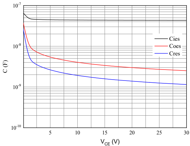
Figure 9. Capacitance characteristic
