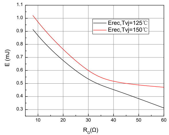
Fig. 8. Switching losses of Diode I_F=75\text{A} , V_{CE}=400\text{V}
