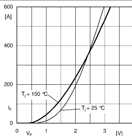
Fig. 10: Typ. FRD diode forward charact., incl. R_{CC'}+EE'
