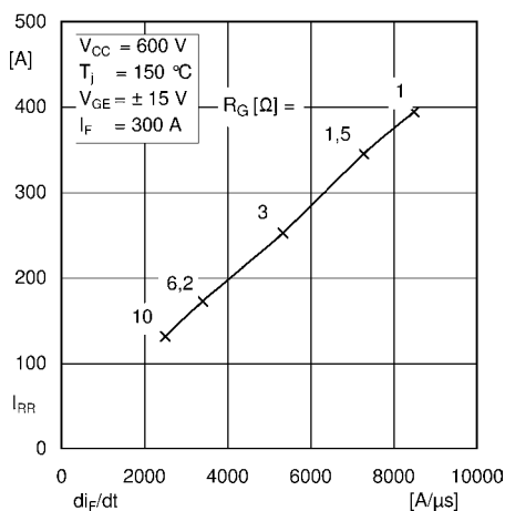
Fig. 11: FRD diode peak reverse recovery current
