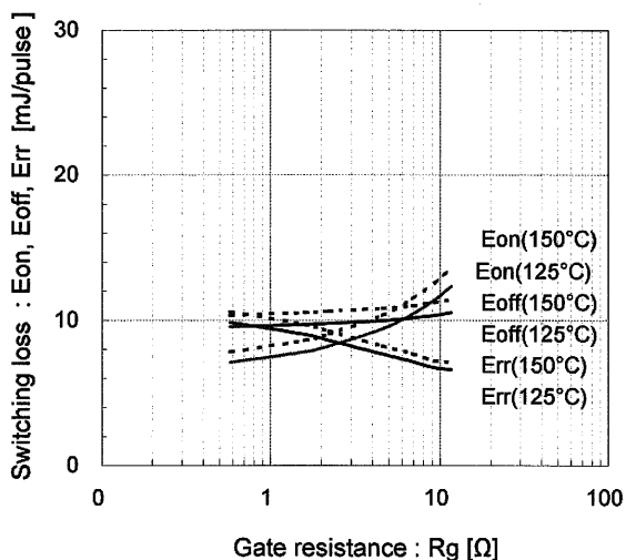
Switching loss vs. gate resistance (typ.) V_{CC}=600V , I_C=100A , V_{GE}=\pm 15V
