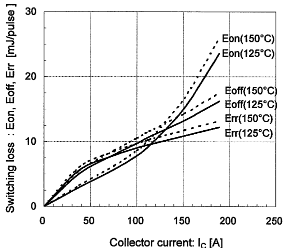
Switching loss vs. Collector current (typ.) V_{CC}=600V , V_{GE}=\pm 15V , R_g=1.6\Omega
