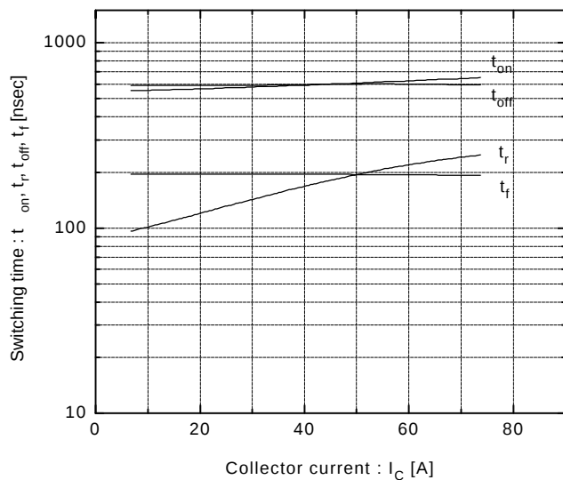
Switching time vs. Collector current V_{CC} = 300V, R_G = 51\Omega, V_{GE} = \pm 15V, T_J = 25^\circ\text{C}
