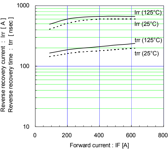
Reverse recovery characteristics (typ.) Vcc=900V, VGE=±15V, Rg=1.1Ω
