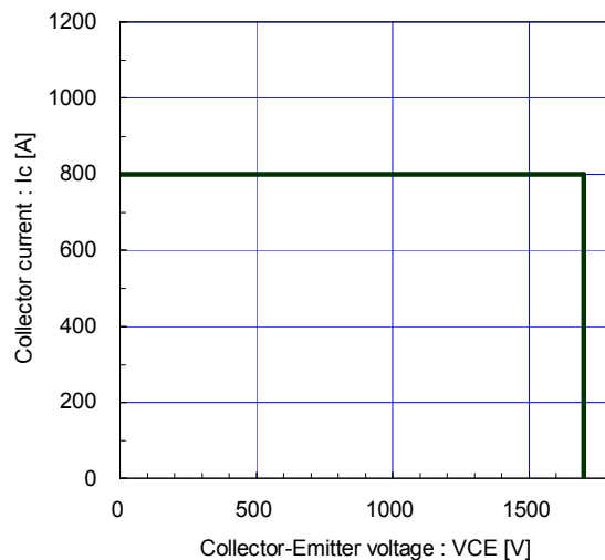
Reverse bias safe operating area (max.) +VGE=15V, -VGE ≤ 15V, Rg ≥ 1.1Ω, Tj ≤ 125°C
