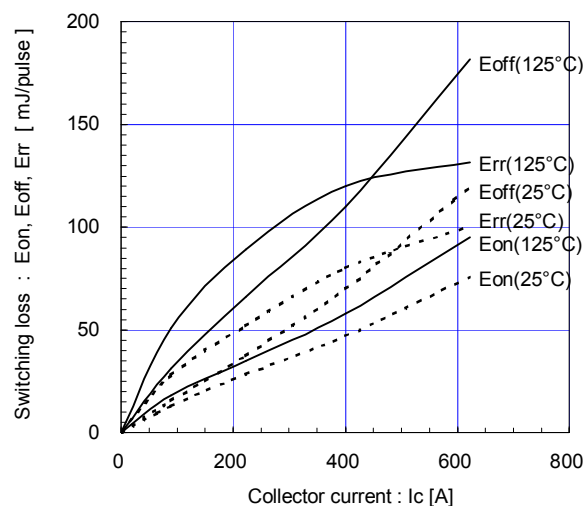
Switching loss vs. Collector current (typ.) Vcc=900V, VGE=±15V, Rg=1.1Ω
