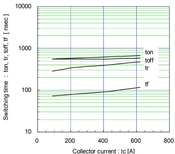
Switching time vs. Collector current (typ.) Vcc=900V, VGE=±15V, Rg=1.1Ω, Tj= 25°C
