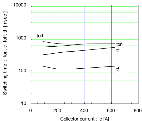
Switching time vs. Collector current (typ.) Vcc=900V, VGE=±15V, Rg=1.1Ω, Tj=125°C
