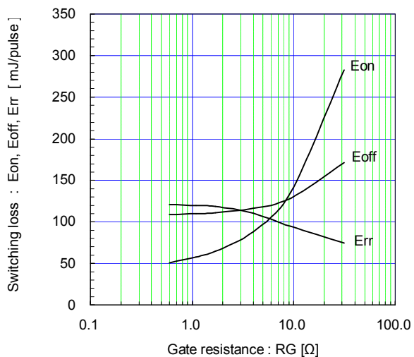
Switching loss vs. Gate resistance (typ.) Vcc=900V, Ic=400A, VGE=±15V, Tj= 125°C
