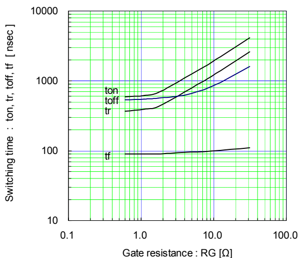
Switching time vs. Gate resistance (typ.) Vcc=900V, Ic=400A, VGE=±15V, Tj= 25°C
