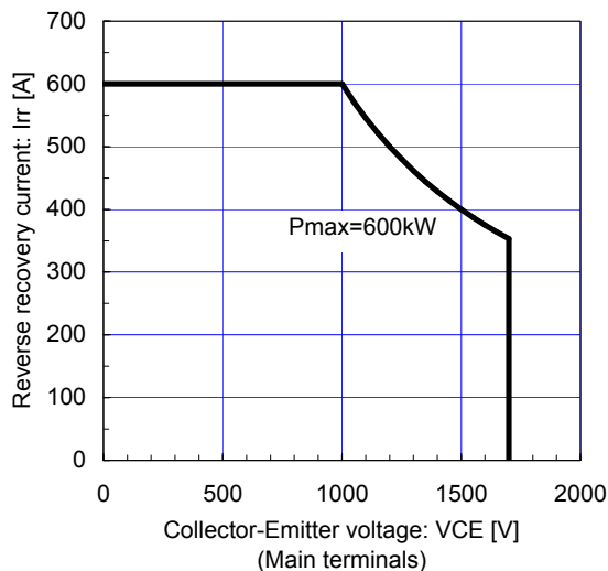
FWD safe operating area (max.) (a) Tj=150°C
