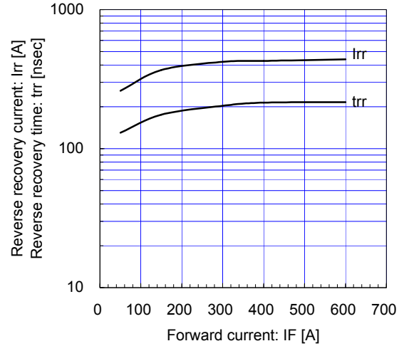
Reverse Recovery Characteristics (typ.) (a) Vcc=900V, VGE=±15V, Rg_on=4.7Ω, Tj=125°C
