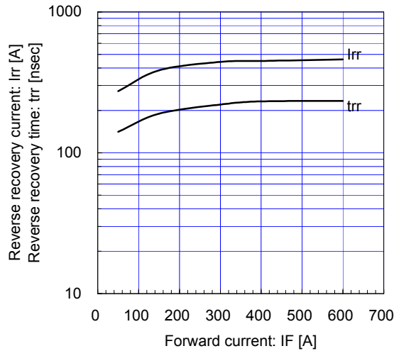
Reverse Recovery Characteristics (typ.) (a) Vcc=900V, VGE=±15V, Rg_on=4.7Ω, Tj=150°C
