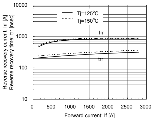
Reverse Recovery Characteristics (typ.) Vcc=600V, Vge=±15V, Rg=1Ω, Tj=125°C, 150°C
