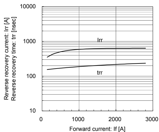
Reverse Recovery Characteristics (typ.) Vcc=600V, Vge=±15V, Rg=1Ω, Tj=25°C
