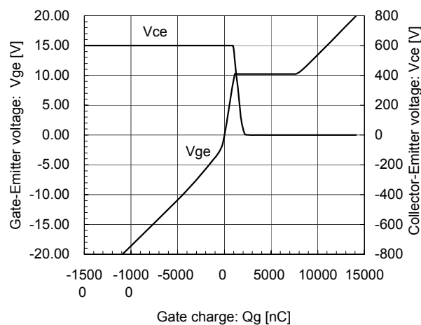
Dynamic Gate Charge (typ.) Vcc=600V, Ic=1400A, Tj= 25°C
