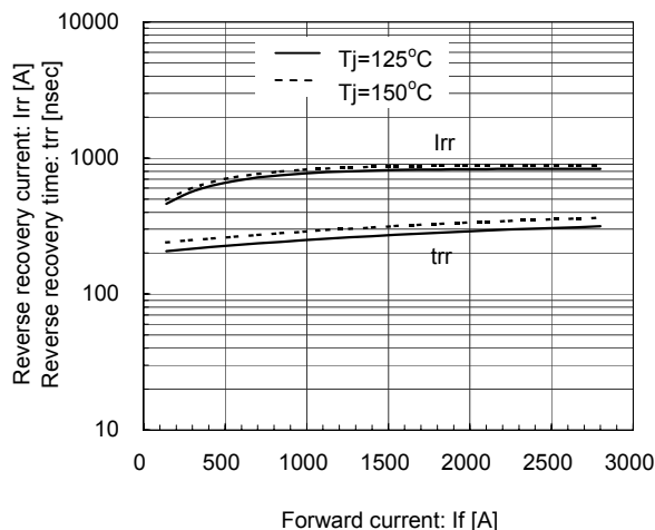
Reverse Recovery Characteristics (typ.) Vcc=600V, Vge=±15V, Rg=1Ω, Tj=125°C, 150°C
