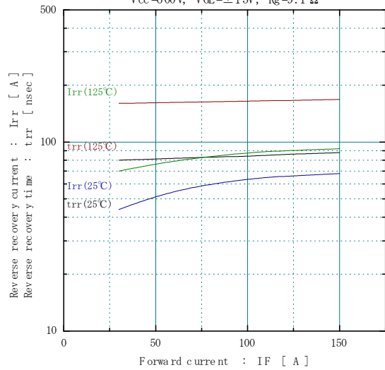
Reverse recovery characteristics (typ.) Vcc=600V, VGE=±15V, Rg=9.1 Ω
